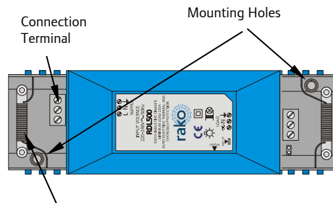
Fig. 2. Termination Area
