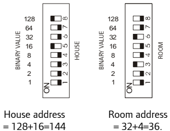
Fig. 4. Addressing Switches
