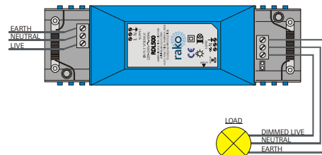
Fig. 3. Connection Detail
