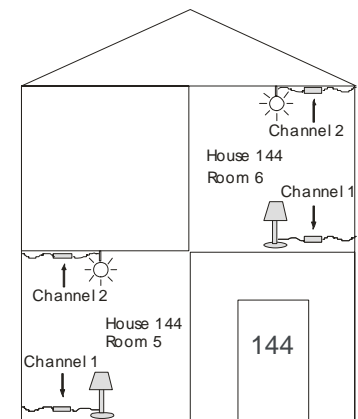
Fig. 5. Addressing Example
