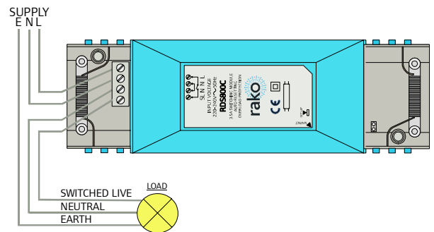
Fig 3. Connection Detail
