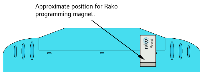
Fig 9. Set-up Magnet Positioning
