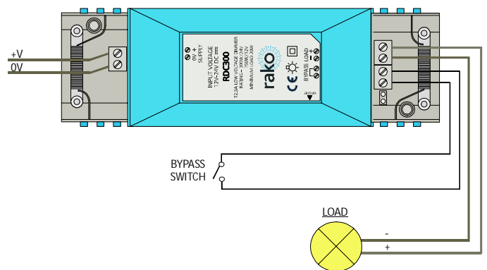
Fig 3. Connection Detail
