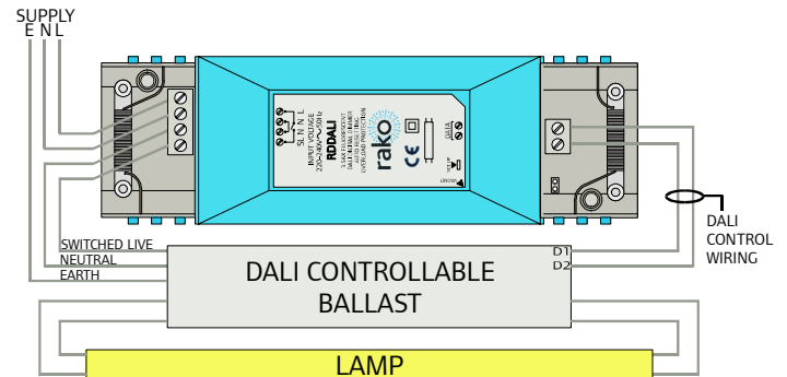
Fig 3. Connection Detail
