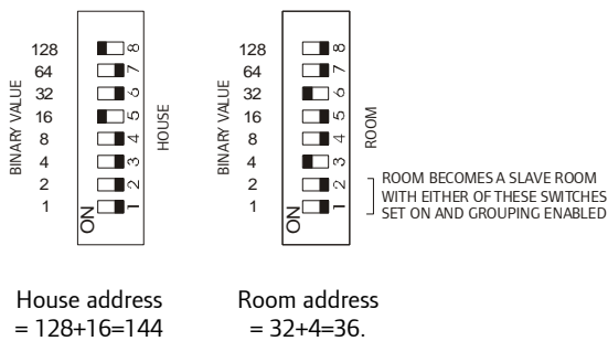
Fig 5. Addressing Switches
