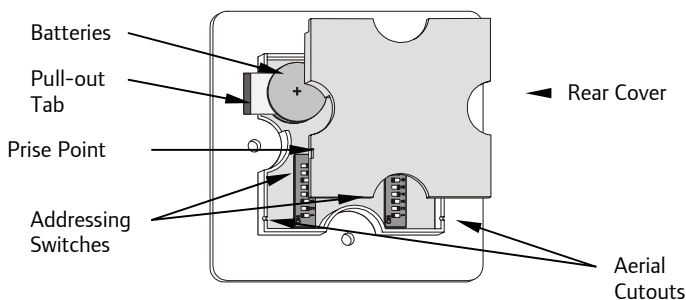
Fig 2. Rear View of PCB Retainer and Rear Cover
