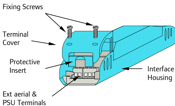
Fig 1. Front View of Components
