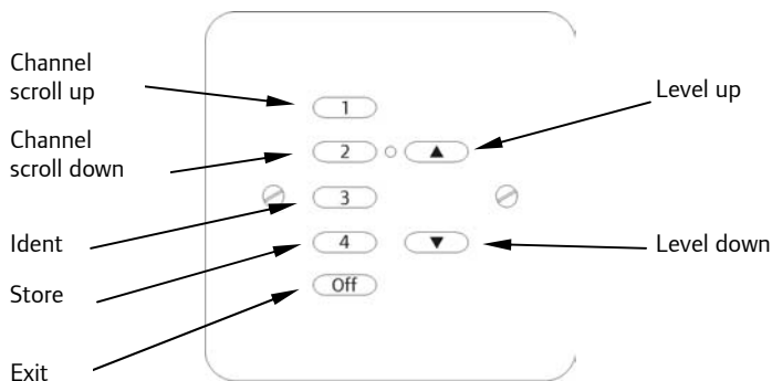
Fig 4. Wall-plate buttons in programming mode
