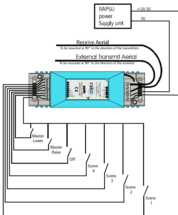
Fig 2. Connection Detail
