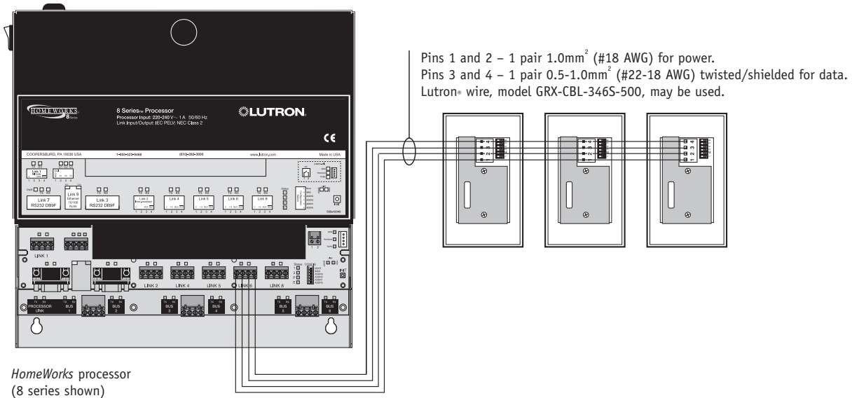
Figure 2 – wiring diagram
